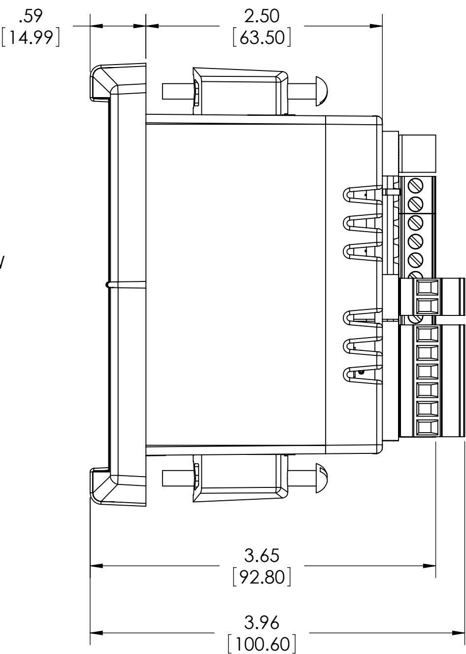
SIDE VIEW
