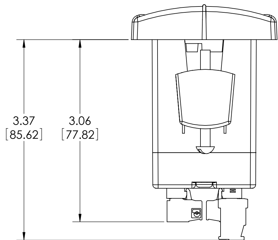
BOTTOM VIEW
