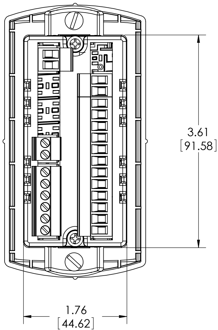
REAR VIEW
