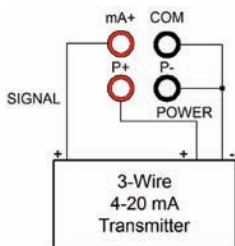
Wiring for a 3 wire external 4-20 mA transmitter.
