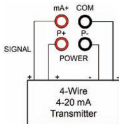
Wiring for a 4 wire external 4-20 mA transmitter.
